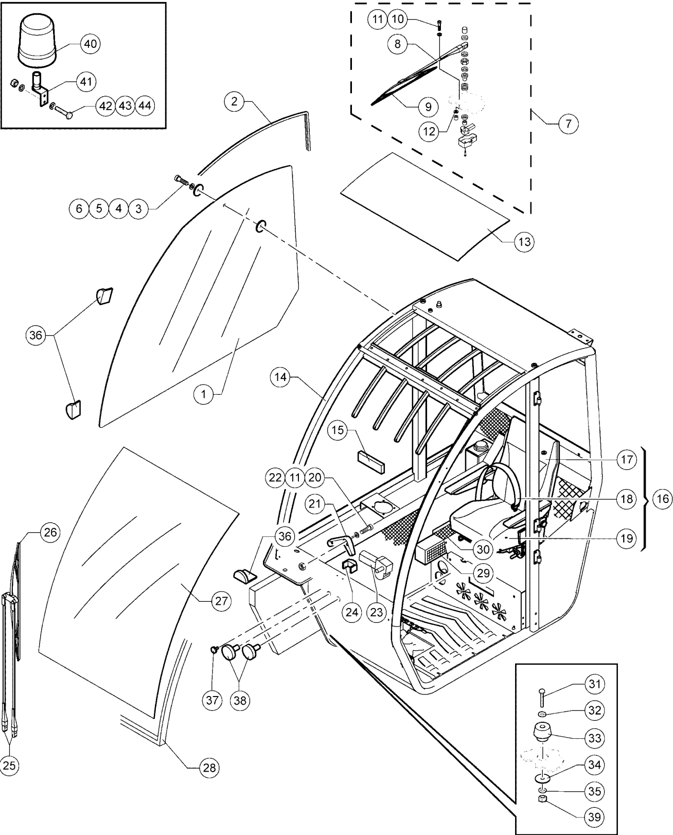
401.1 605522 Closed Cabin, View 1
